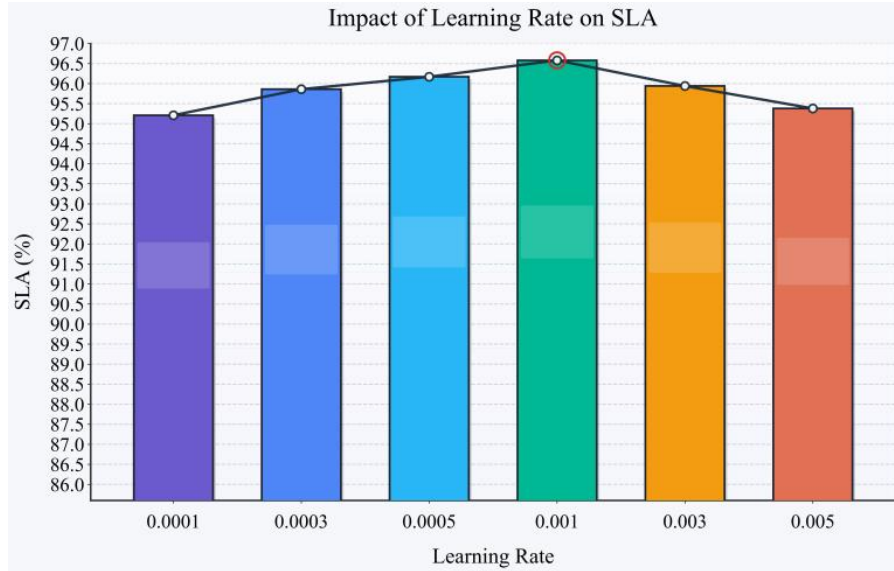
Figure 2. The impact of learning rate sensitivity on SLA
