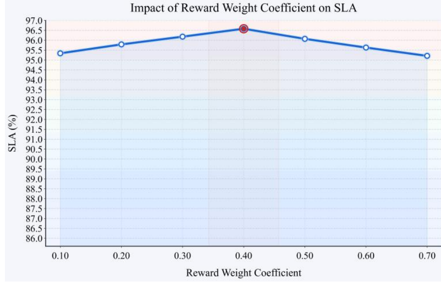
Figure 3. Impact of Reward Weighting Coefficient Sensitivity on SLA
