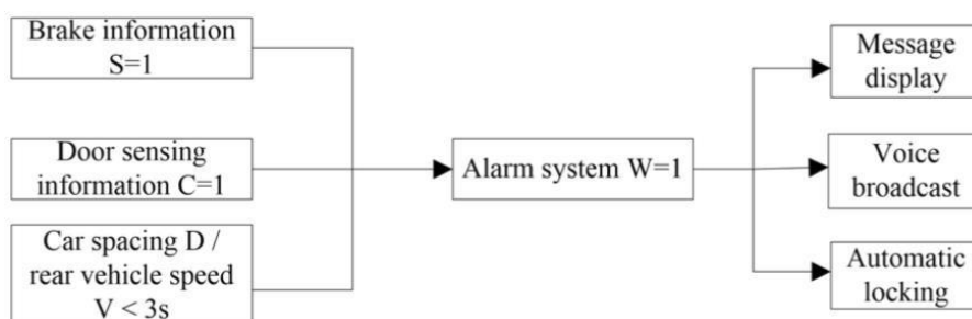
Figure 3. Information processing judgment flow chart
