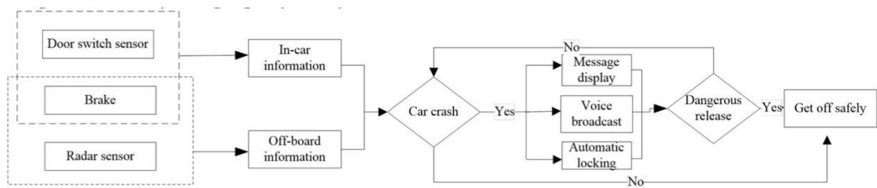
Figure 2. Structure of the car door collision avoidance system
