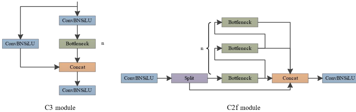
Figure 2. C3 module and C2f module structures
