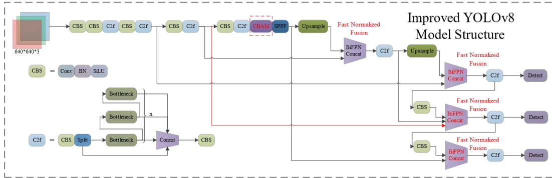
Figure 7. Improved YOLOv8 model structure
