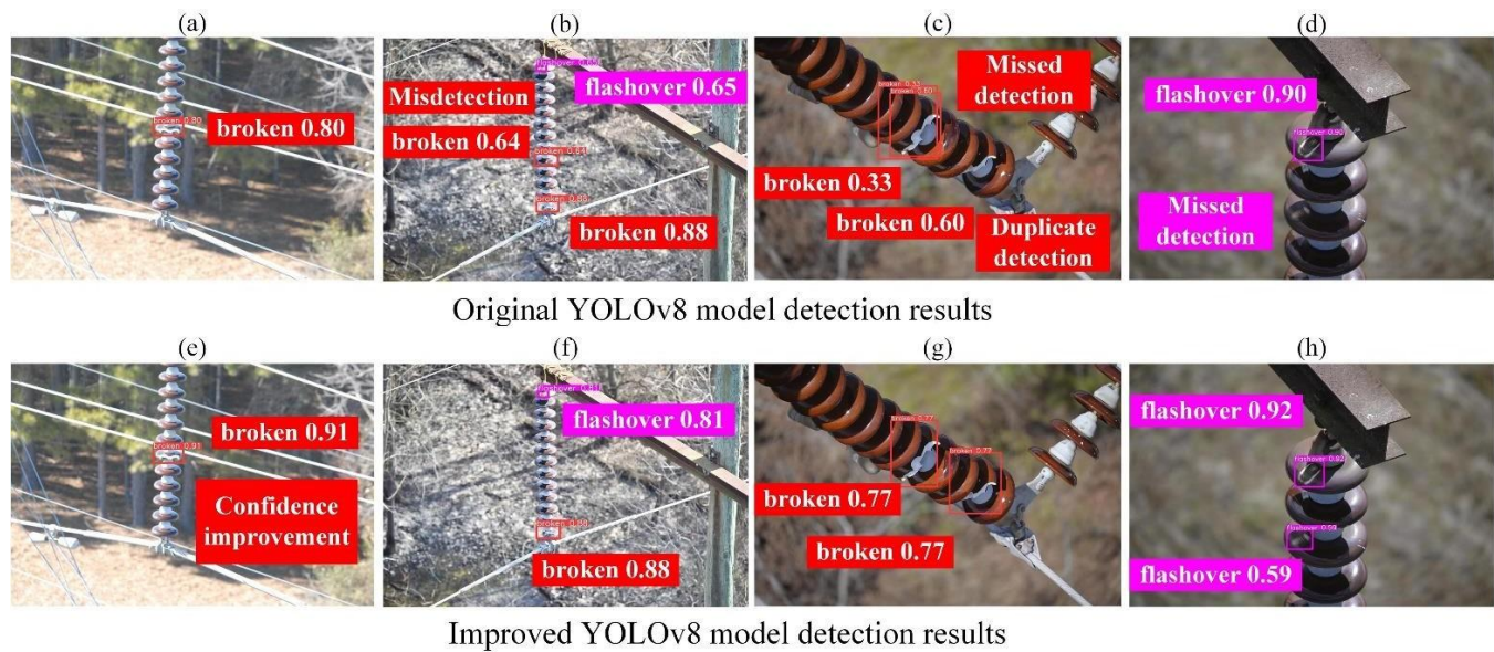
Figure 8. Comparison of original YOLOv8 model and improved YOLOv8 model detection results The detection results in Figure 8 (a) and Figure 8 (e) show that the improved YOLOv8 model can improve the confidence of object detection, and it can be seen that the confidence in detecting broken insulators has increased by 0.11. The improved YOLOv8 model has improved the feature extraction ability, making object detection more accurate; The detection results in Figure 8 (b) and Figure 8 (f) indicate that the original YOLOv8 model identified intact insulators as broken insulators, resulting in misdetection. However, the improved YOLOv8 model accurately identified whether insulators had broken faults, effectively avoiding misdetection; The detection results in Figures 8 (c) and 8 (g) indicate that the original YOLOv8 model duplicatedly detects a single object and cannot detect broken insulators with a large occluded area when detecting broken insulators. However, the improved YOLOv8 model can extract the features of the occluded insulator image and accurately identify the insulators with broken faults; The detection results in Figure 8 (d) and Figure 8 (h) indicate that the original YOLOv8 model missed detection when detecting insulation components that were shaded and had flashover faults, while the improved YOLOv8 model weakened the influence of shadows on feature extraction and fusion, effectively improving the accuracy of insulation component fault recognition. From Figure 8, it can be seen that the improved YOLOv8 model has stronger feature extraction ability, performs better in distinguishing similar features, integrates multi-scale features more thoroughly, has stronger ability to detect small objects, and has lower miss detection and misdetection rates. Even in complex outdoor natural environments, it has good detection performance, good robustness and generalization, and can meet the requirements of unmanned inspection. In order to objectively verify the effectiveness of the improved YOLOv8 model, this article conducted comparative experiments with mainstream object detection models using the same dataset in the same experimental environment.
