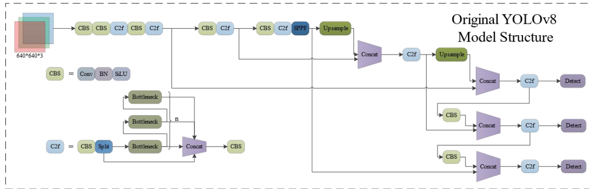
Figure 1. Original YOLOv8 model structure
