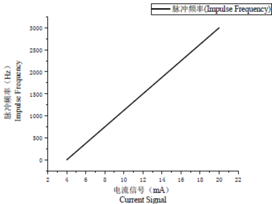
Fig 8. Frequency current diagram
