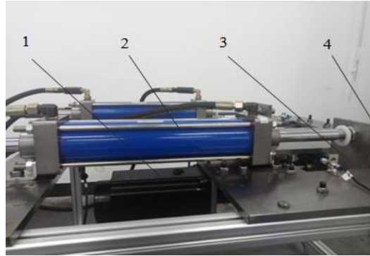
Fig 3. Working platform of metering pump
