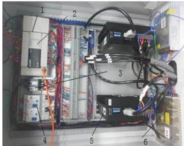
Fig 4. Electrical control cabinet
