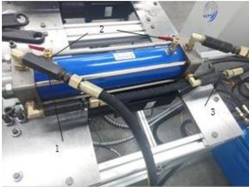
Fig 7. Piping system diagram after commissioning 1—Inlet check valve, 2—Exhaust valve, 3—Drain check valve
