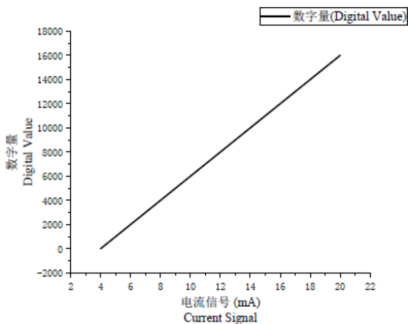
Fig 9. Digital quantity current diagram
