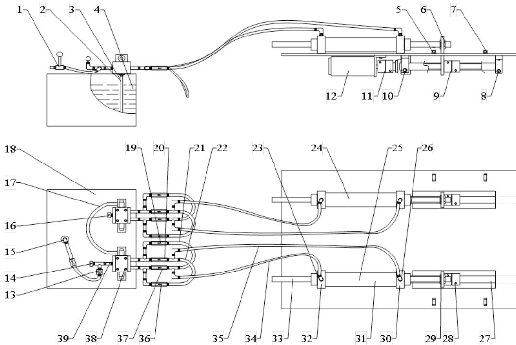
Fig 2. The experimental device
