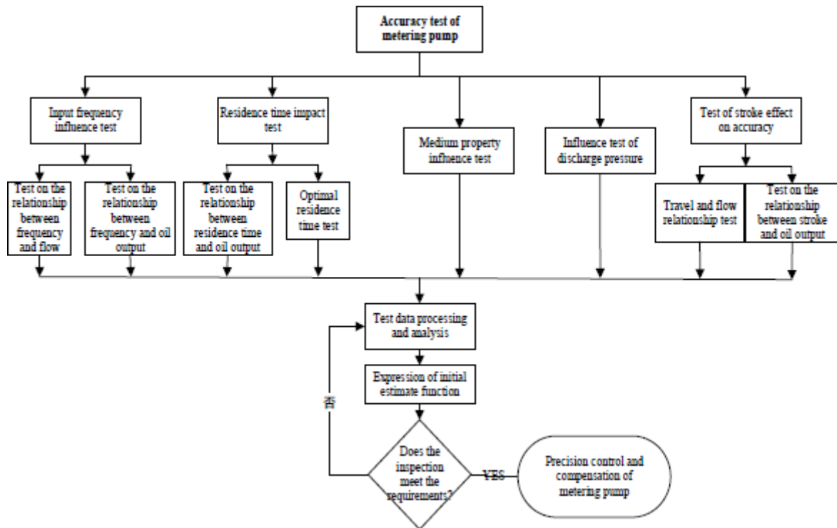
Fig 10. Technical route of experimental research
