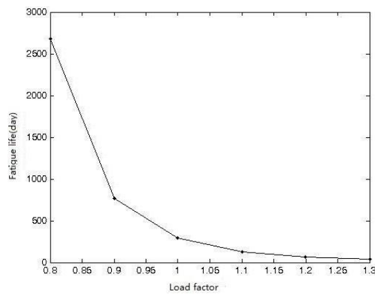
Fig 2. Influence of load factor on fatigue life curve
