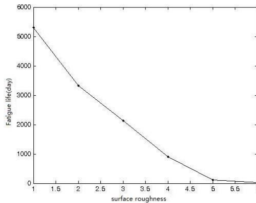
Fig 3. Influence of surface roughness on fatigue life curve
