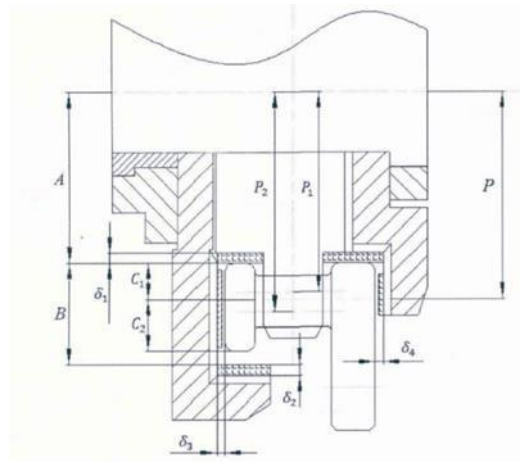
Fig 1. Installation diagram of traveling wheel and pin row guide shoe
