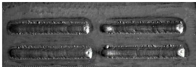
Fig 2. Laser cladding after optimizing process parameters
